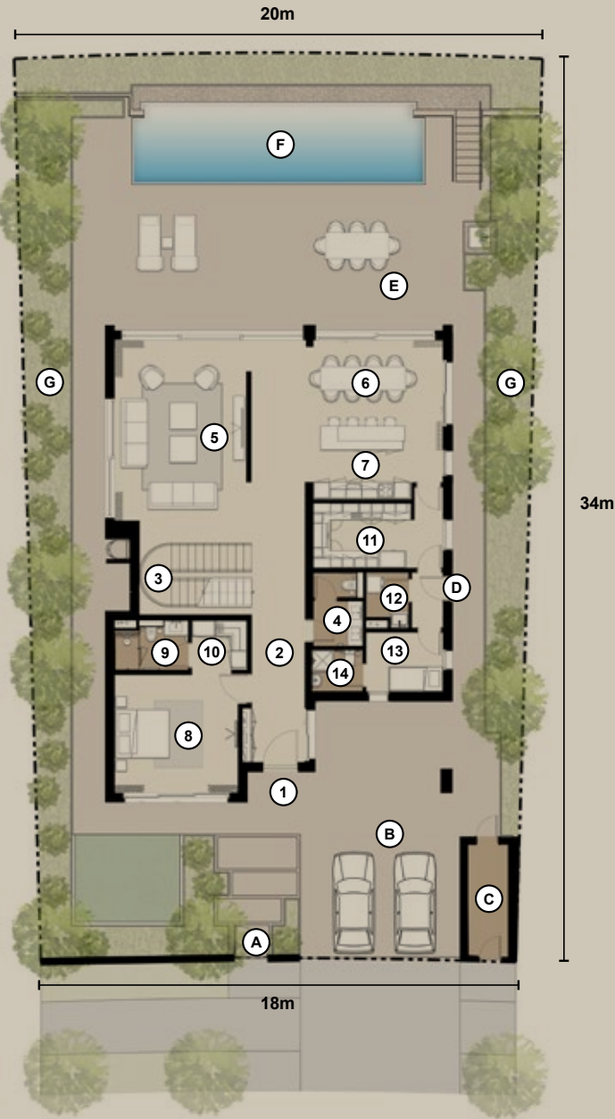
GROUND FLOOR
